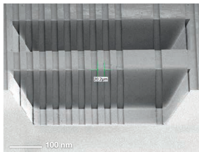
High depth of focus exposure of KOH etched cavities with a depth of 150 μm Source: EVG
