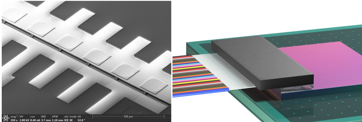
Nanoimprint of wafer-level optics on silicon photonics wafer (Left) for Teramount PhotonicPlug's scalable fiber connectivity (Right).
